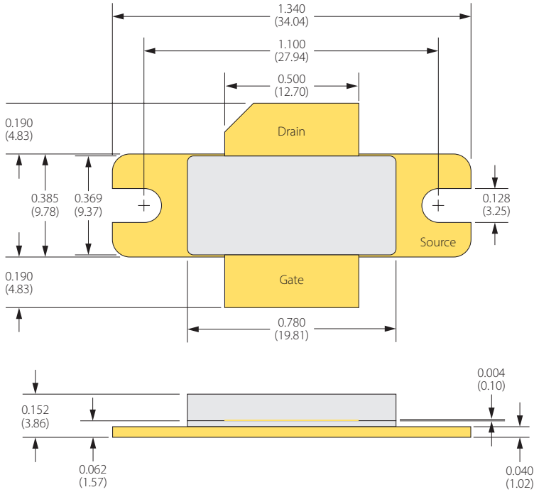
BOLT-DOWN FLANGE OPTION IGN1090M800
