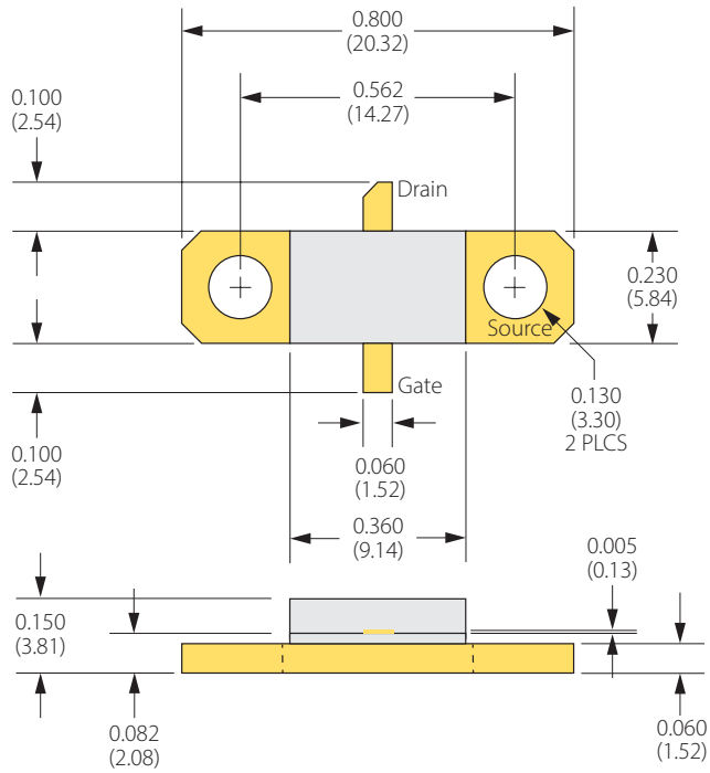
BOLT-DOWN FLANGE OPTION IGN3135L12
