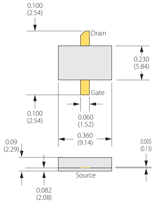
EARLESS FLANGE OPTION IGN3135L12S
