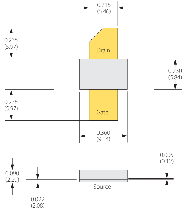
EARLESS FLANGE OPTION IGN2932M75S
