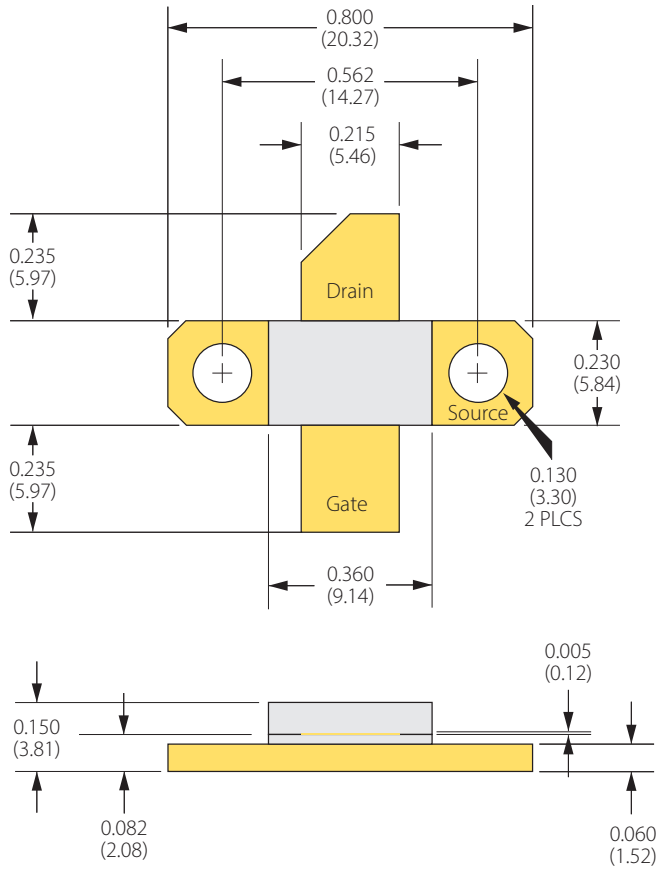
BOLT-DOWN FLANGE OPTION IGN2932M75
