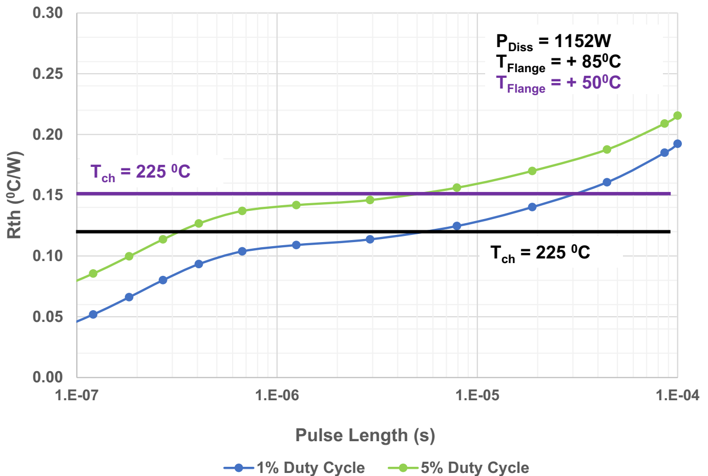
Figure 4. (Data obtained by FEA analysis)
