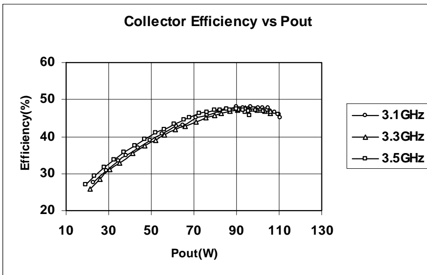
Typical values, Vcb = 36 V, 150µs RF pulse, 10% duty cycle
