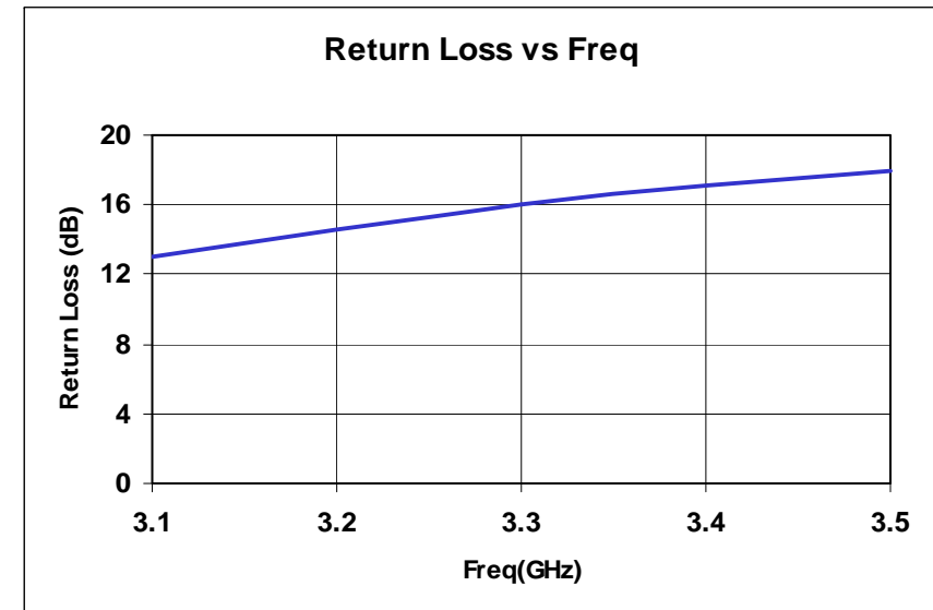
Typical values, Vcb = 36 V, 150µs RF pulse, 10% duty cycle, Pin = 14W
