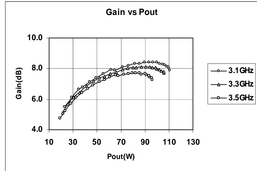
Typical values, Vcb = 36 V, 150µs RF pulse, 10% duty cycle
