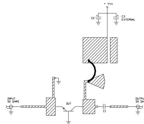
ELECTRICAL SCHEMATIC
